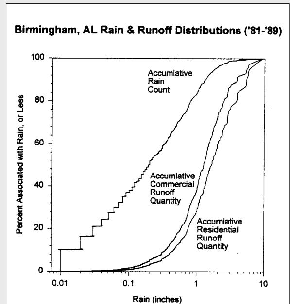
Figure 2. Rainfall and runoff distribution for Birmingham, AL
