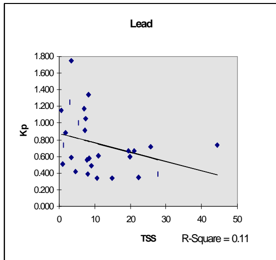
Figure 3. K_p as a function of TSS.
