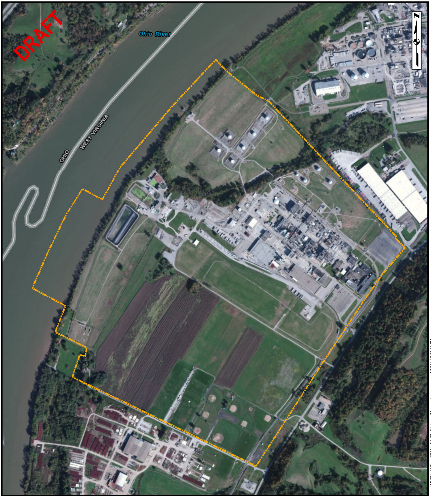
Figure B-2: Site Layout Map
