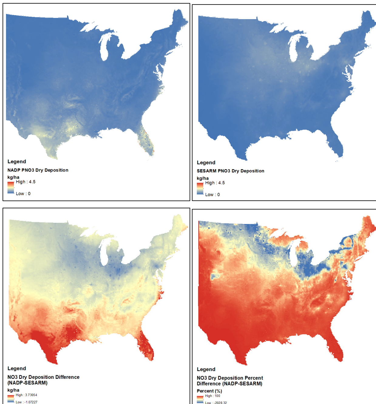
Figure 7-41. Plots of Total Annual Particulate \text{NO}_3^+ Dry Deposition. NADP Dry Deposition (top left), SESARM Dry Deposition (top right), Difference (bottom left), Percent Difference 103 (bottom right).
