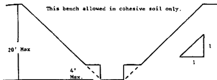
SINGLE BENCH
