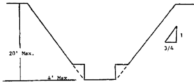
SIMPLE BENCH
