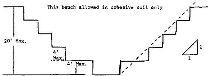
MULTIPLE BENCH
