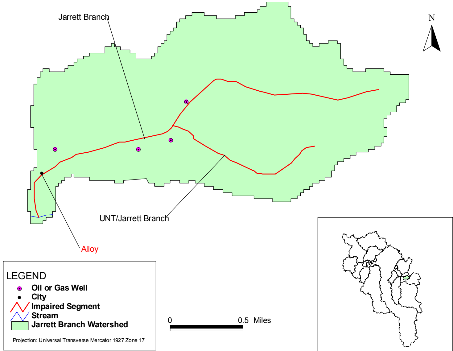
Figure A-8-7. Oil and gas wells in the Jarrett Branch watershed
