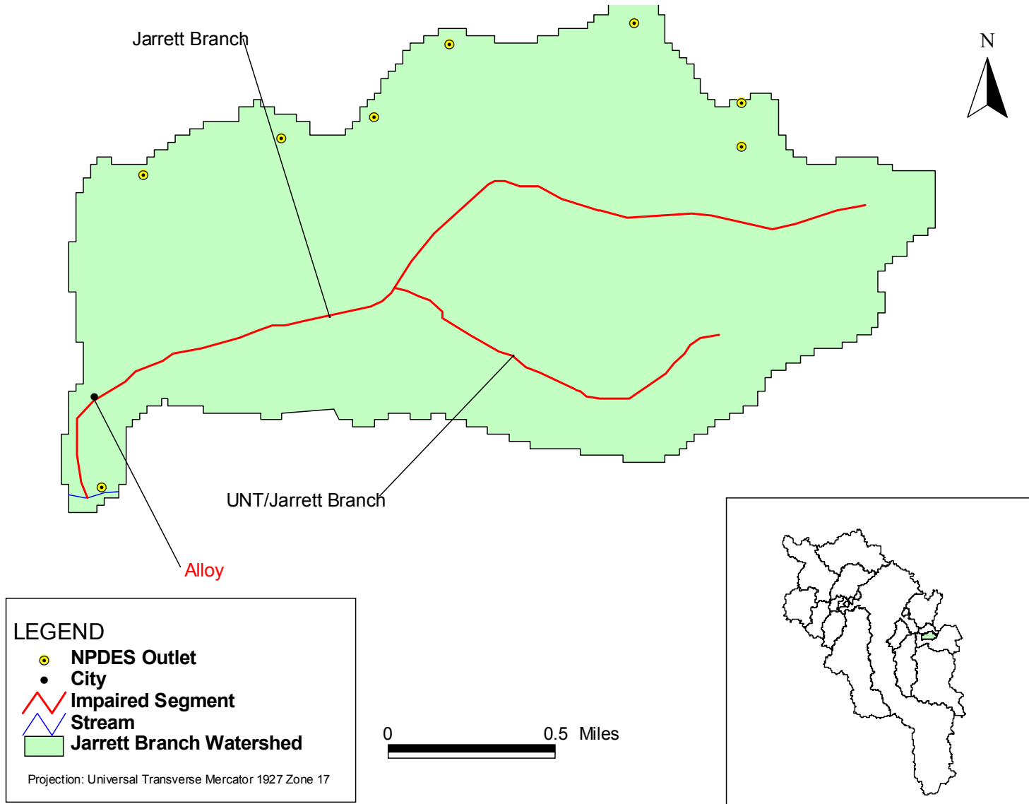
Figure A-8-5. NPDES outlets in the Jarrett Branch watershed
