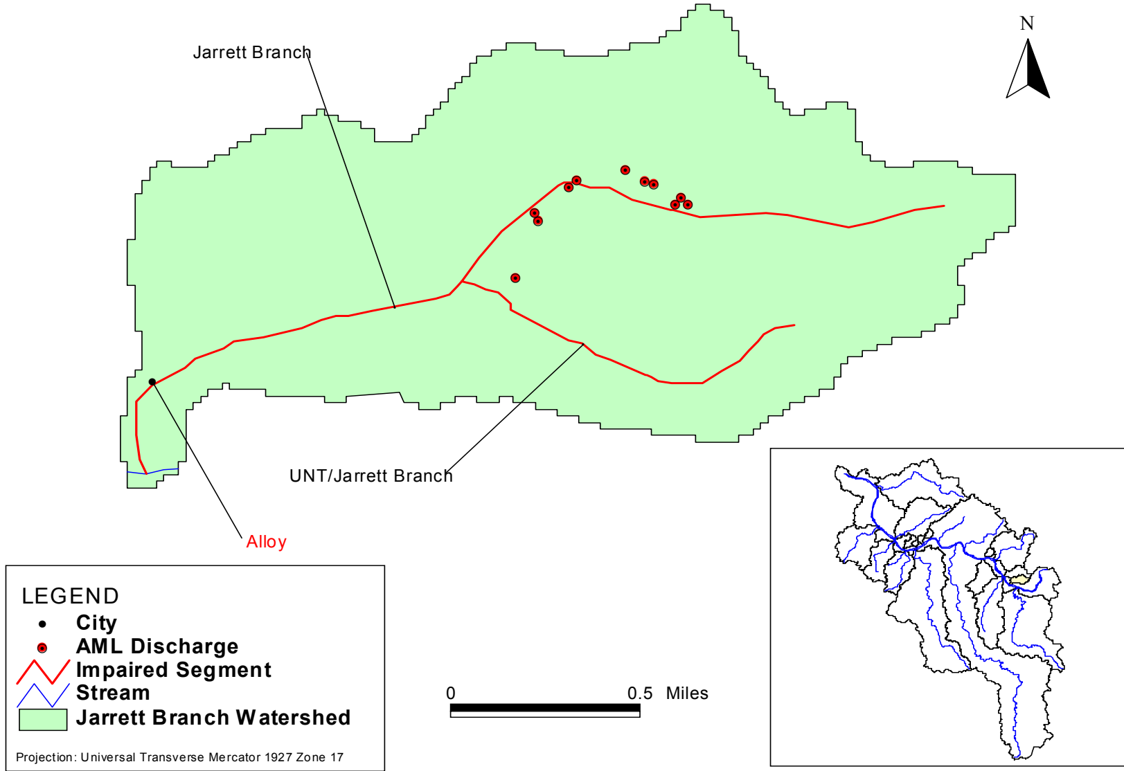
Figure A-8-6. Abandoned mine lands in the Jarrett Branch watershed
