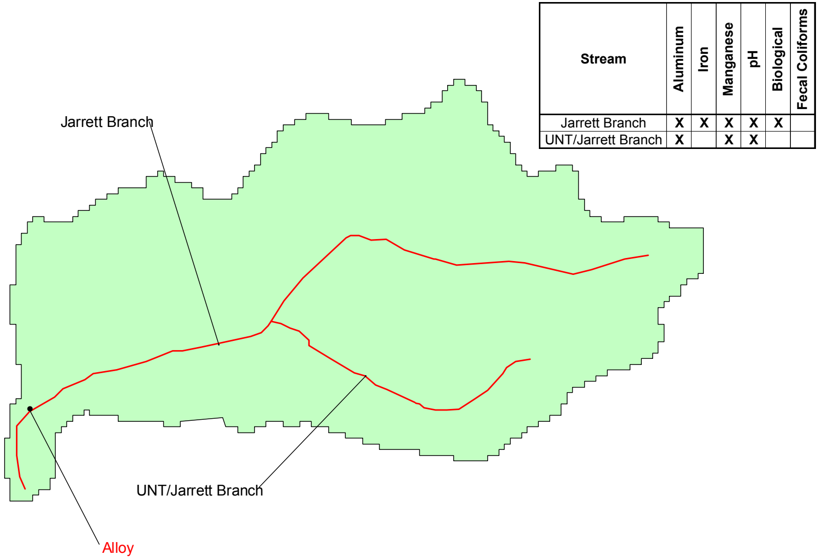
Figure A-8-3. Impaired waterbodies in the Jarrett Branch watershed
