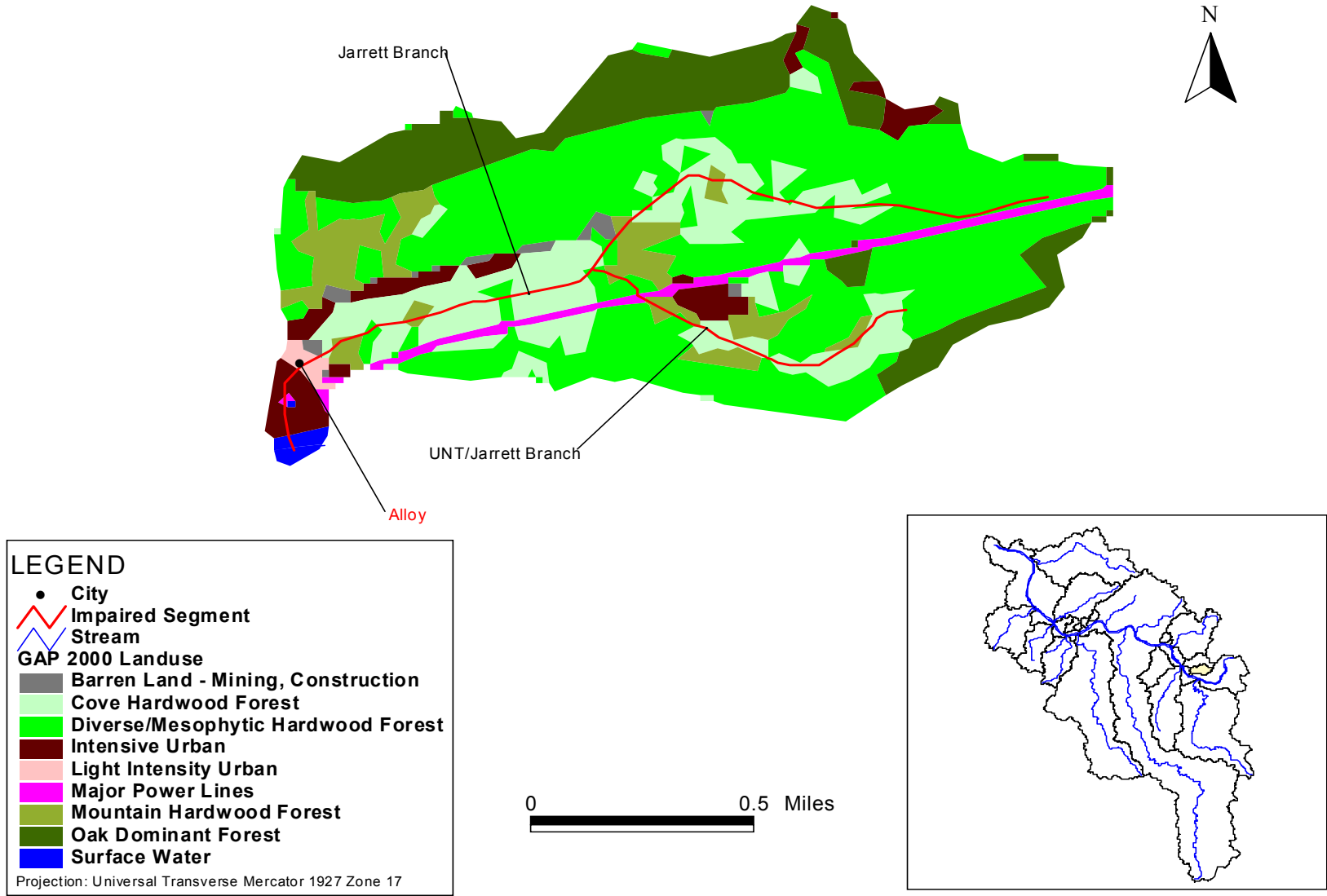
Figure A-8-2. Land use distribution in the Jarrett Branch watershed
