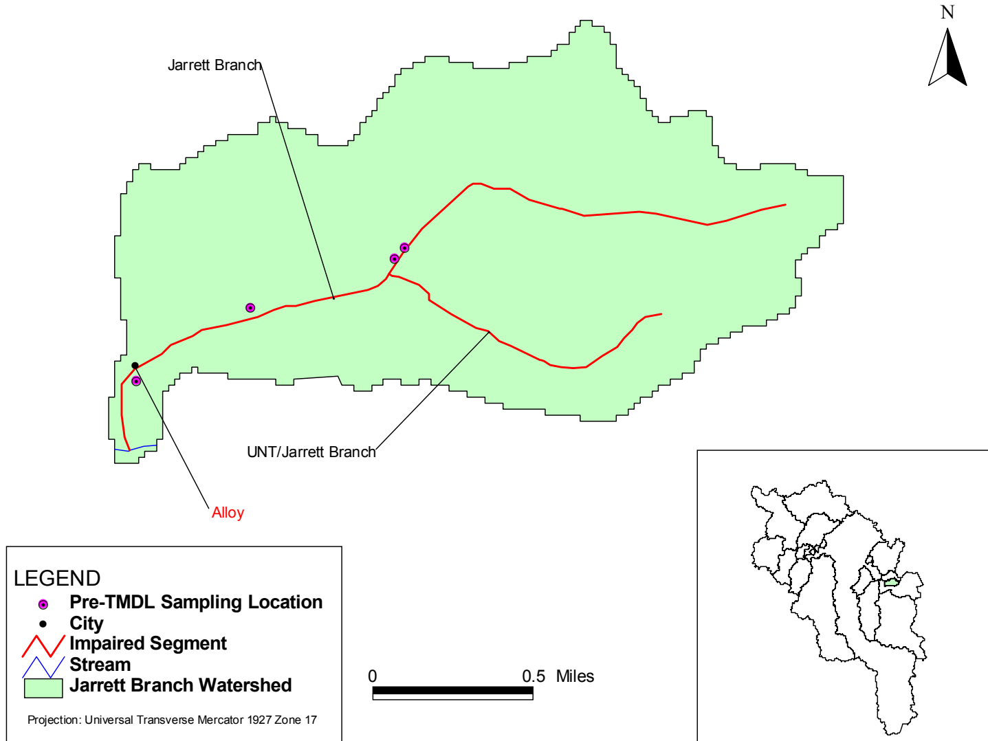
Figure A-8-4. Pre-TMDL monitoring stations in the Jarrett Branch watershed
