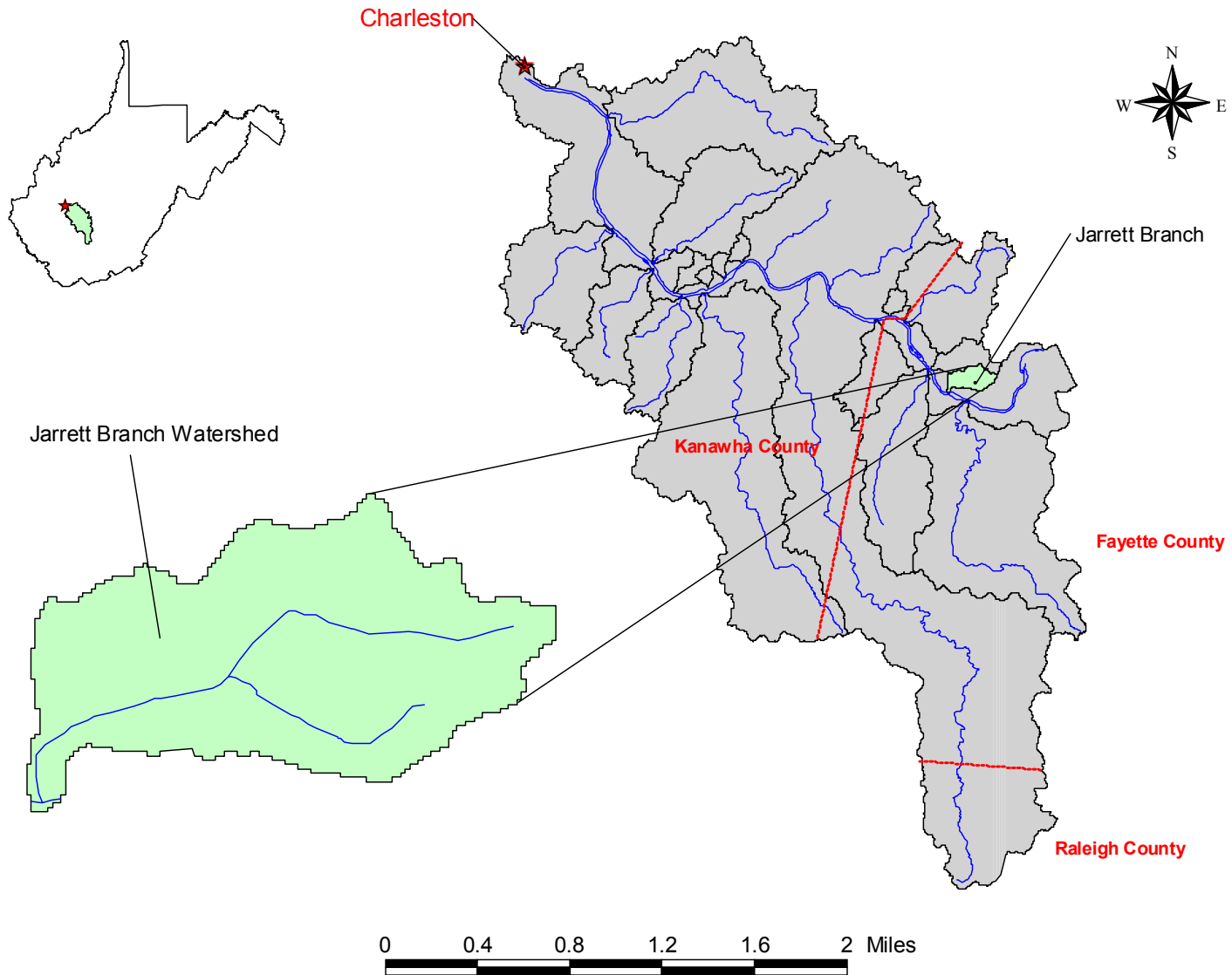
Figure A-8-1. Location of the Jarrett Branch watershed
