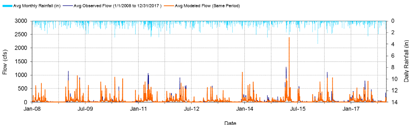
Figure 6-1. Comparison of simulated and observed flow from January 2008 to December 2017 for East Fork/Twelvepole Creek (WV-OT-45)
