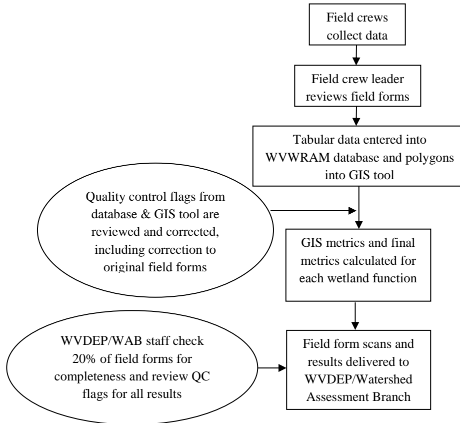
Figure 2. Data management process. Squares depict step processes and ovals depict quality assurance checks.
