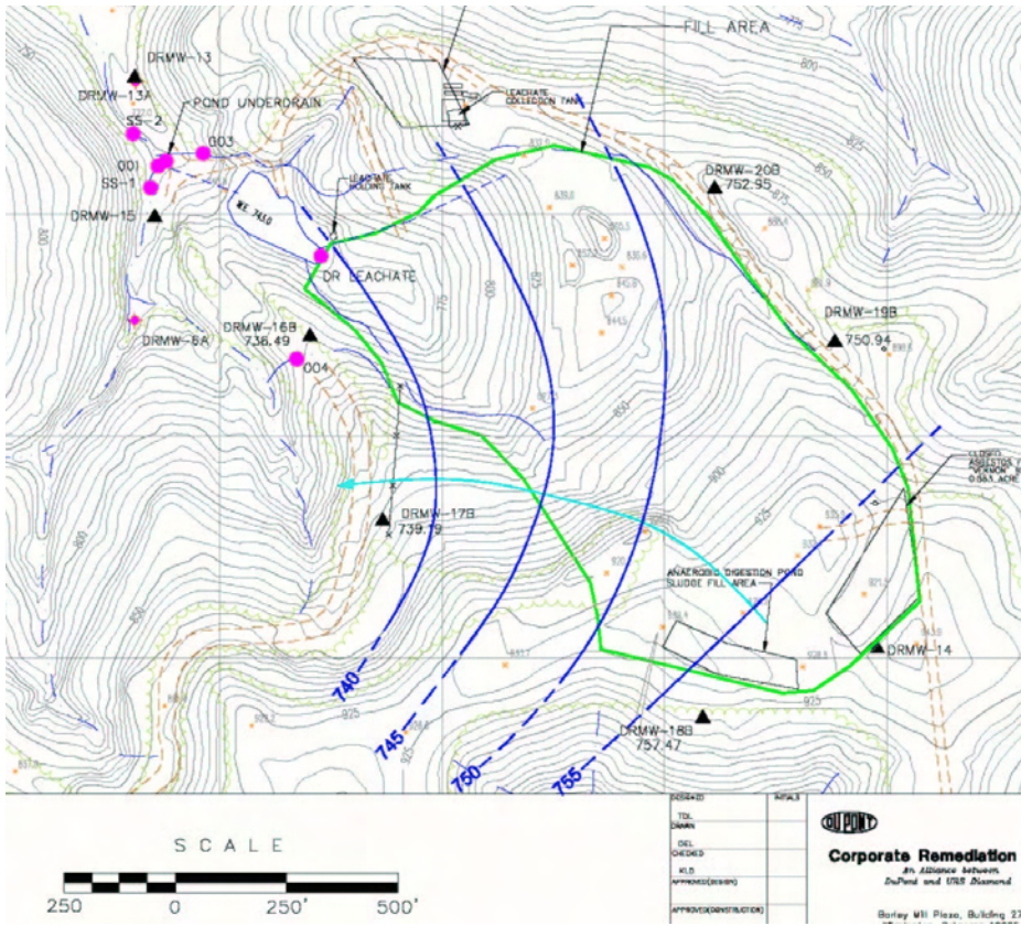
Figure 2.7: Dry Run Zone A Top-of-Groundwater Map.
