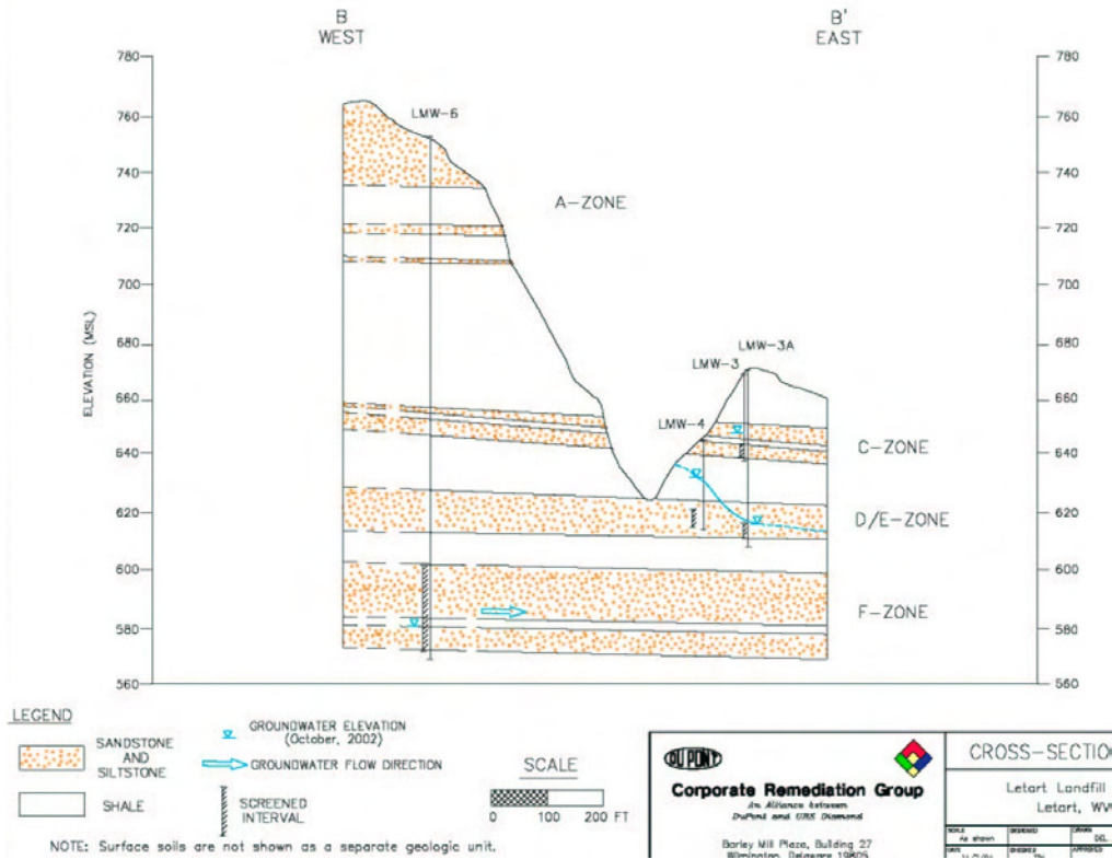
Figure 3.5: Letart Landfill Geological Cross-Section B-B'.
