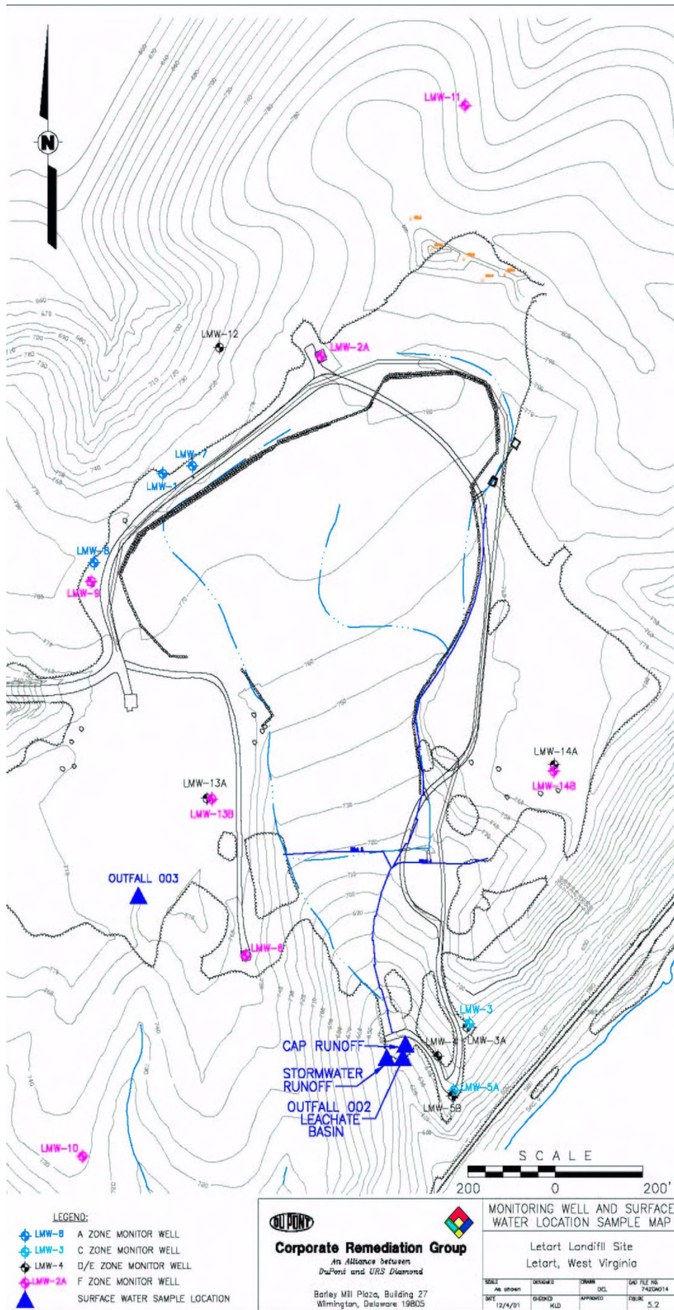
Figure 3.2: Letart Landfill and Sampling Points.
