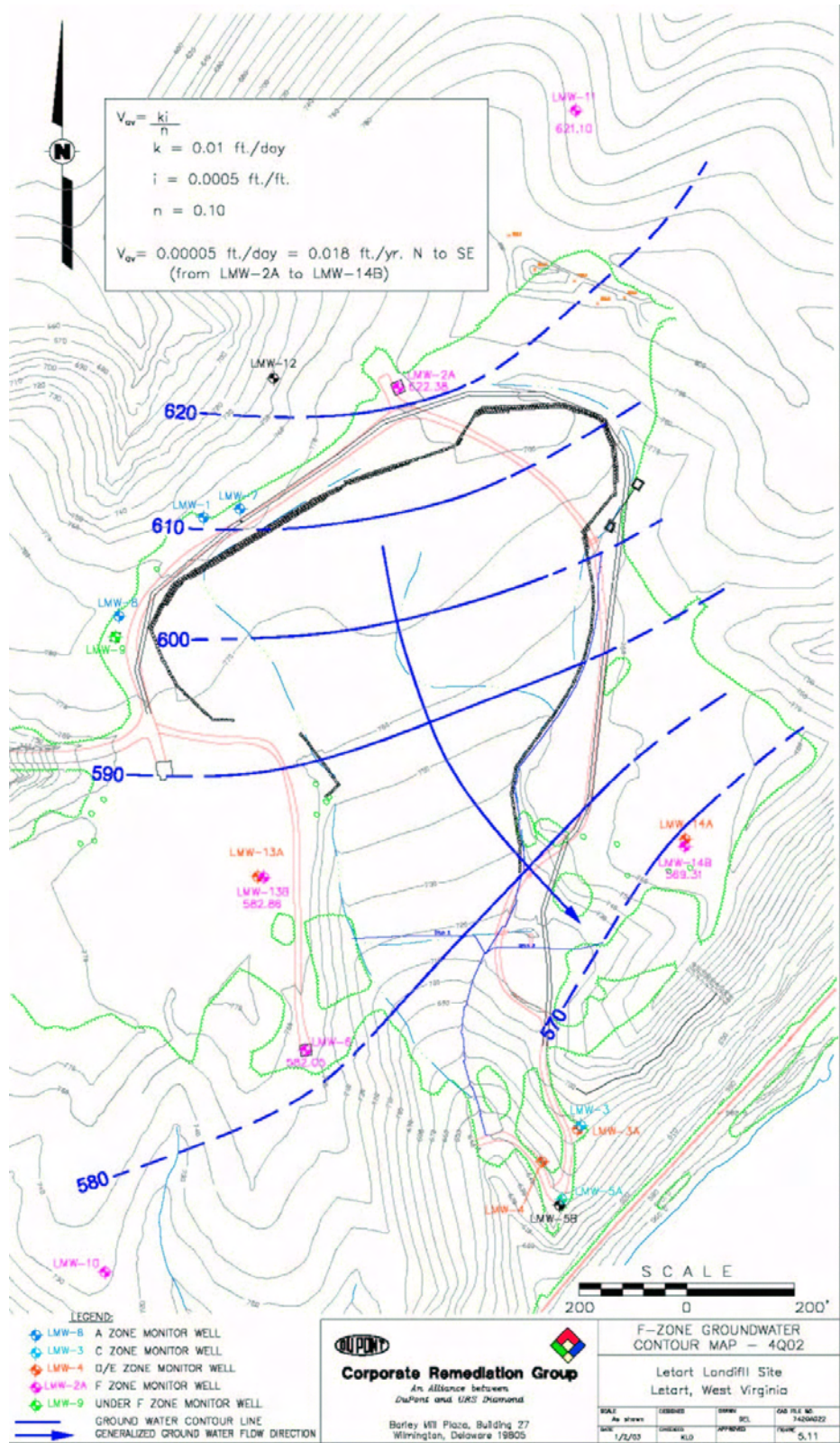
Figure 3.9: Letart Landfill Zone F Top-of-Groundwater Map.
