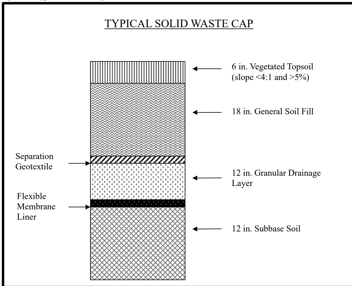
Figure F-4: Typical Solid Waste Cap
