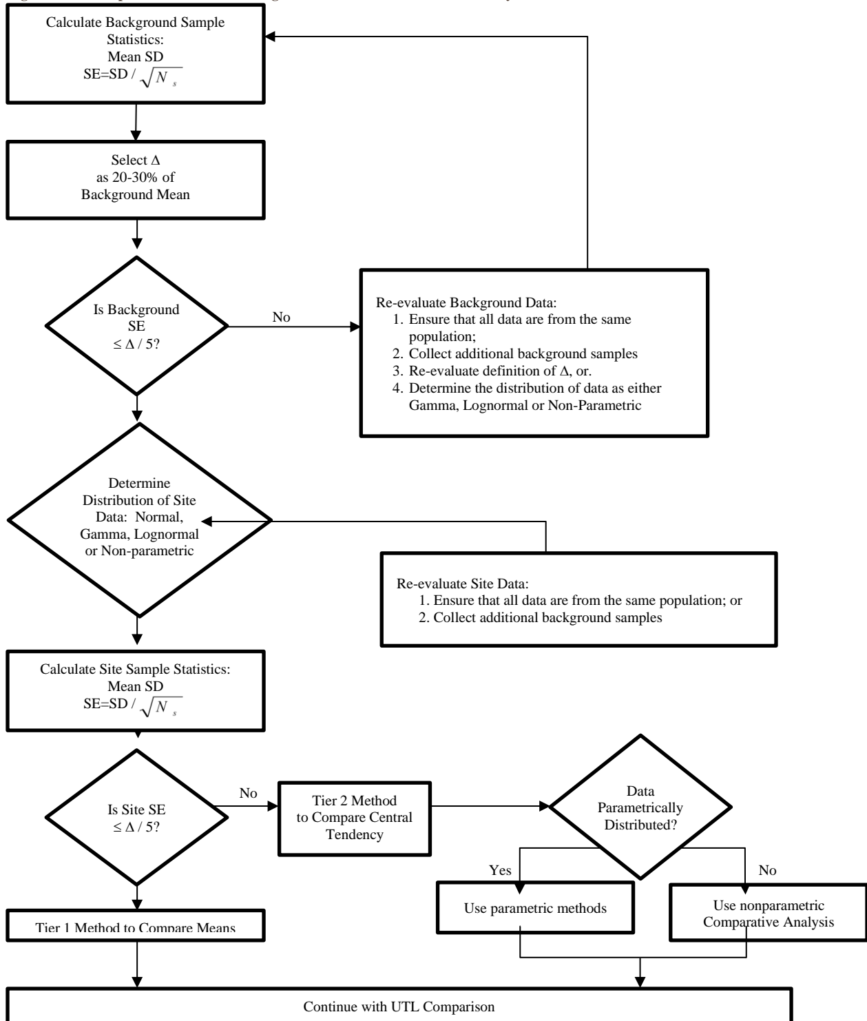
Figure A-4: Comparison of Site and Background Measures of Central Tendency
