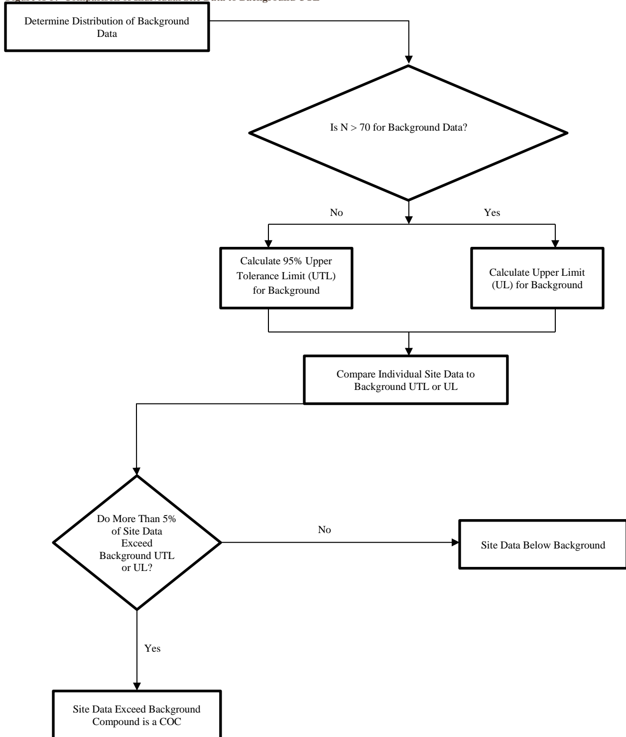
Figure A-5: Comparison of Individual Site Data to Background UTL
